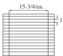
15 Cell Arrangement Max Cell size 15-3/4 x 1 x 8-1/4" 2 Short Partitions - 14 Long Partitions
