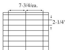
14 Cell Arrangement Max Cell size 7-3/4 x 2-1/4 x 8-1/4" 3 Short Partitions - 7 Long Partitions
