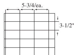
15 Cell Arrangement Max Cell size 5-3/4 x 3-1/2 x 8-1/4" 4 Short Partitions - 4 Long Partitions
