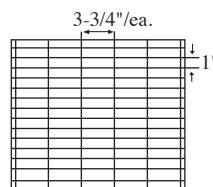
75 Cell Arrangement Max Cell size 3-3/4 x 1 x 8-1/4" 6 Short Partitions - 14 Long Partitions
