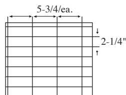
21 Cell Arrangement Max Cell size 5-3/4 x 2-1/4 x 8-1/4" 4 Short Partitions - 7 Long Partitions
