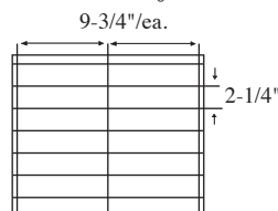
14 Cell Arrangement Max Cell size 9-3/4 x 2-1/4 x 8-1/4" 3 Short Partitions - 7 Long Partitions
