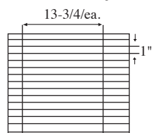
15 Cell Arrangement Max Cell size 13-3/4 x 1 x 8-1/4" 2 Short Partitions - 14 Long Partitions
