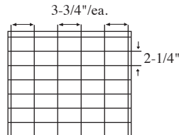
35 Cell Arrangement Max Cell size 3-3/4 x 2-1/4 x 8-1/4" 6 Short Partitions - 7 Long Partitions
