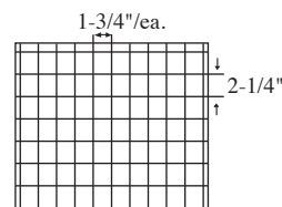
70 Cell Arrangement Max Cell size 1-3/4 x 2-1/4 x 8-1/4" 11 Short Partitions - 7 Long Partitions
