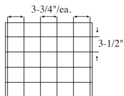
25 Cell Arrangement Max Cell size 3-3/4 x 3-1/2 x 8-1/4" 6 Short Partitions - 14 Long Partitions
