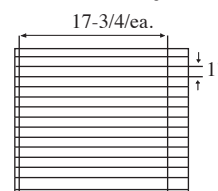
15 Cell Arrangement Max Cell size 17-3/4 x 1 x 8-1/4" 2 Short Partitions - 14 Long Partitions
