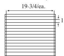
15 Cell Arrangement Max Cell size 19-3/4 x 1 x 8-1/4" 2 Short Partitions - 14 Long Partitions
