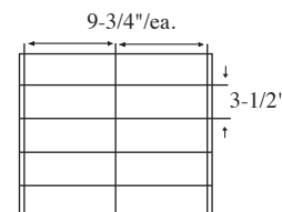
10 Cell Arrangement Max Cell size 9-3/4 x 2-1/4 x 8-1/4" 3 Short Partitions - 4 Long Partitions
