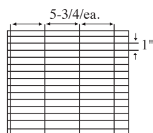
45 Cell Arrangement Max Cell size 5-3/4 x 1 x 8-1/4" 4 Short Partitions - 14 Long Partitions
