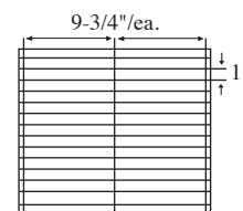
30 Cell Arrangement Max Cell size 9-3/4 x 1 x 8-1/4" 3 Short Partitions - 14 Long Partitions
