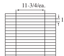
15 Cell Arrangement Max Cell size 11-3/4 x 1 x 8-1/4" 2 Short Partitions - 14 Long Partitions
