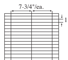
30 Cell Arrangement Max Cell size 7-3/4 x 1 x 8-1/4" 3 Short Partitions - 14 Long Partitions
