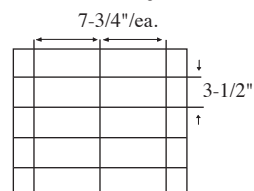
10 Cell Arrangement Max Cell size 7-3/4 x 3-1/2 x 8-1/4" 3 Short Partitions - 4 Long Partitions
