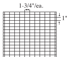
150 Cell Arrangement Max Cell size 1-3/4 x 1 x 8-1/4" 11 Short Partitions - 14 Long Partitions
