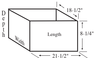
45 Cell Arrangement Max Cell size 5-3/4 x 1 x 8-1/4" 4 Short Partitions - 14 Long Partitions
