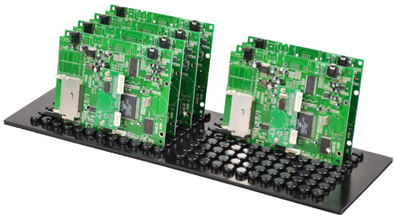
Grid Tray can be customized to be all conductive.
